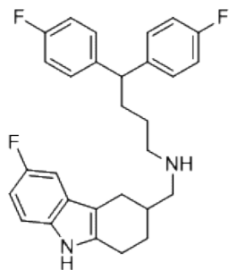
PC-6254201, CDCl 3
